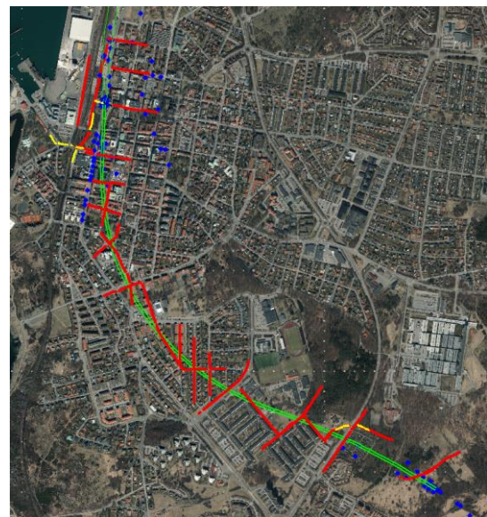
Figure 8 Landstreamer seismic lines carried out within the Varberg railway tunnel project, primarily to identify the bedrock surface and the rock quality.
